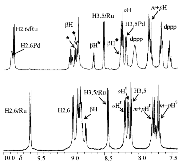
Figure 1. Bottom: Downfield region of the ^1\text{H} NMR spectrum of 6 in \text{CDCl}_3 ( \tau : position 15, \sigma : position 20). Top: The same spectral region after addition of one equivalent of 7 , leading to the quantitative formation of molecular square 10 (pyrrole ( \beta ) resonances labeled with \star and \blacklozenge are coupled to each other in the COSY spectrum).
